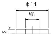
Terminal T9
